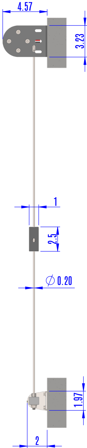
SIDE VIEW
