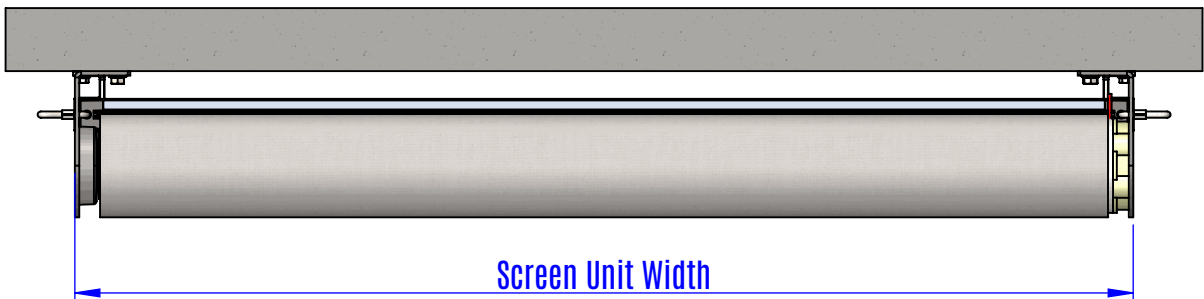
TOP VIEW
