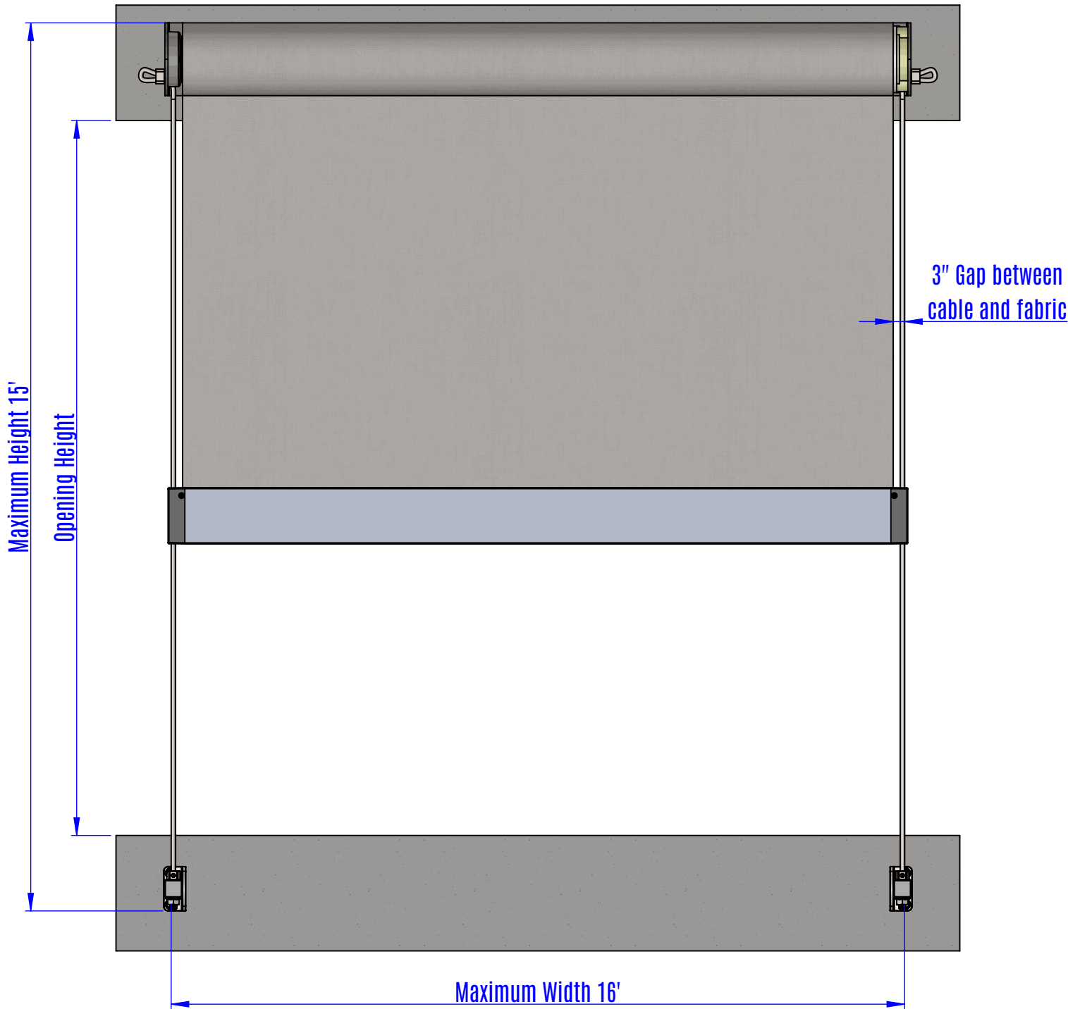
FRONT VIEW
