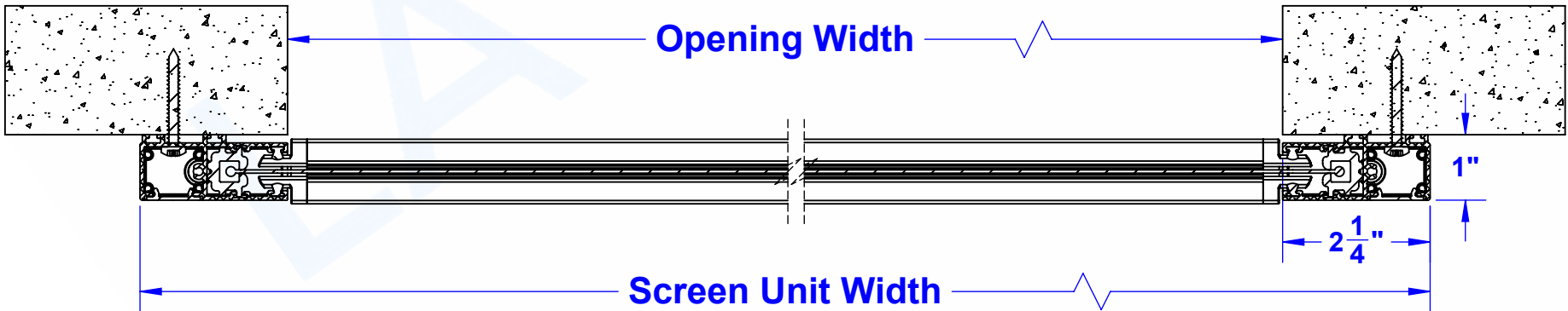
SIDE TRACK DETAIL
