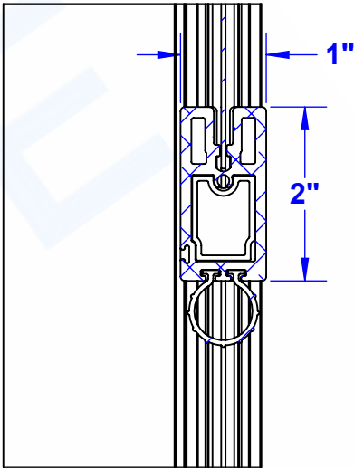
HEM BAR DETAIL
